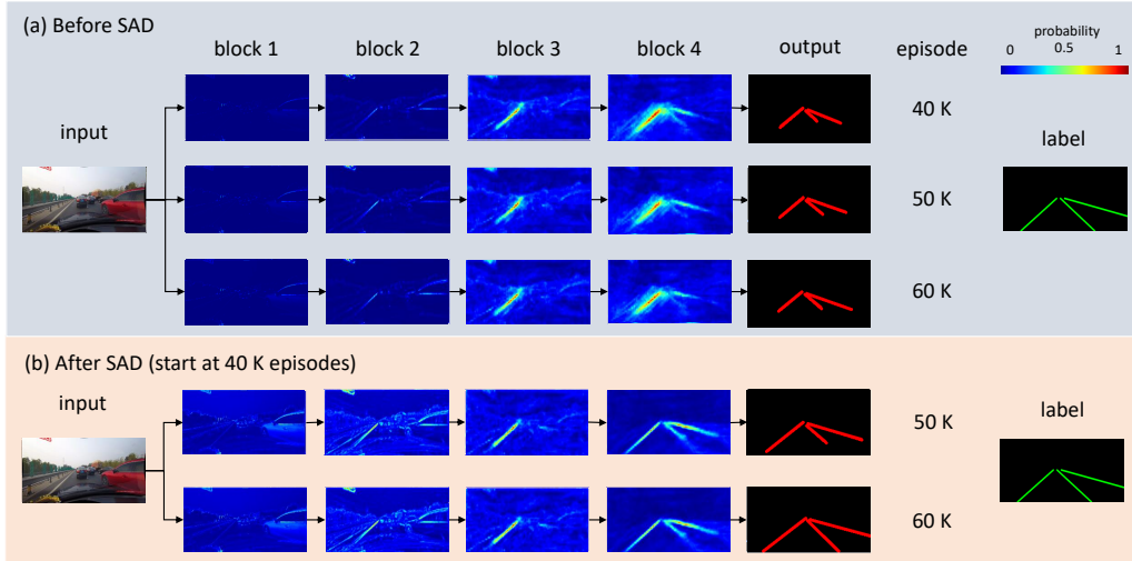
Figure 1. Attention maps of the ENet [20] before and after applying self attention distillation. Here, we extract the attention maps from the four stages/blocks following the design of ENet model. Note that self attention distillation is added in the 40 K episodes.
