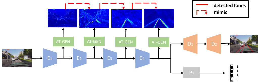
Figure 3. An instantiation of using SAD. E_1 \sim E_4 comprise the encoder of ENet [20], D_1 and D_2 comprise the decoder of ENet. Following [19], we add a small network to predict the existence of lanes, denoted as P_1 . AT-GEN is the attention generator.
