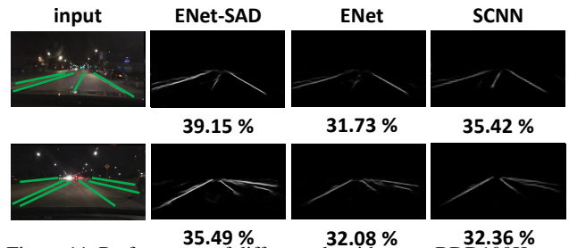
Figure 11. Performance of different algorithms on BDD100K testing set. We visualize the probability maps to better showcase the effect of adding self attention distillation. The brightness of the pixel indicates the probability of this pixel belonging to lanes. The number below each image denotes the pixel accuracy of lanes. Ground-truth lanes are drawn on the input image.
